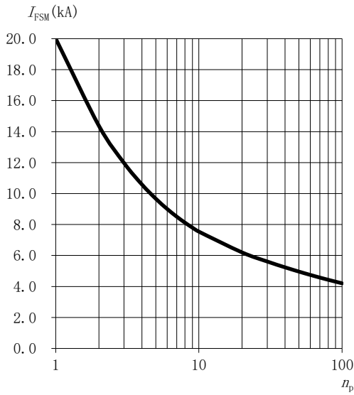
Fig.5: Surge on-state current ( I_{FSM} ) vs. number of pulses ( n_p )
