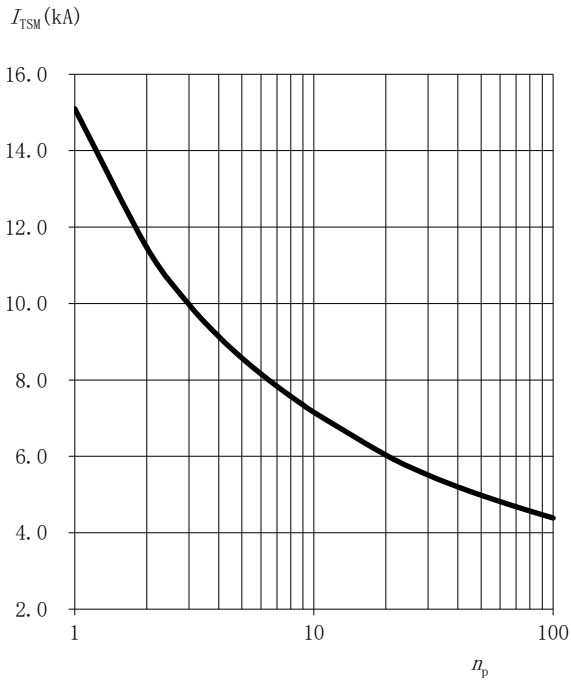
Fig.5: Surge on-state current ( I_{TSM} ) vs. number of pulses ( n_p )
