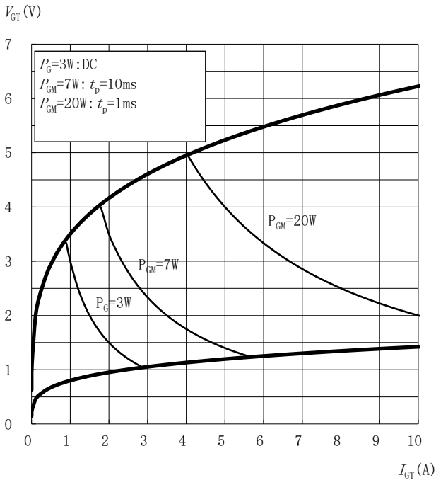
Fig.7: Max. peak gate power loss
