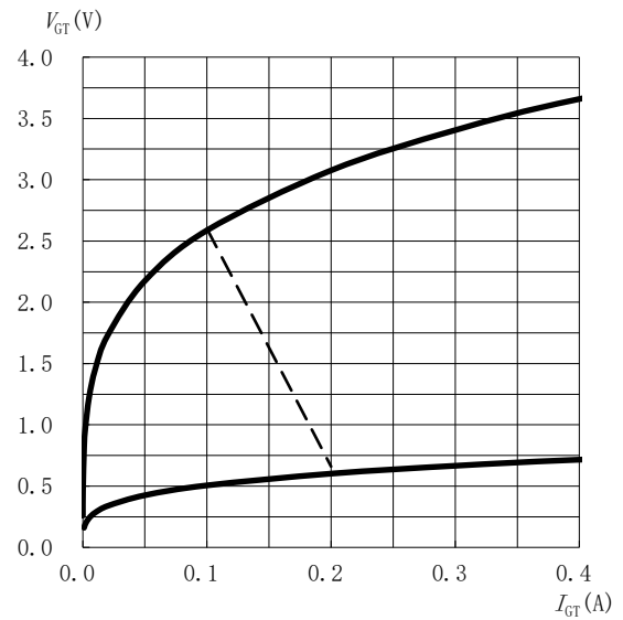
Fig.8: Gate trigger characteristics
