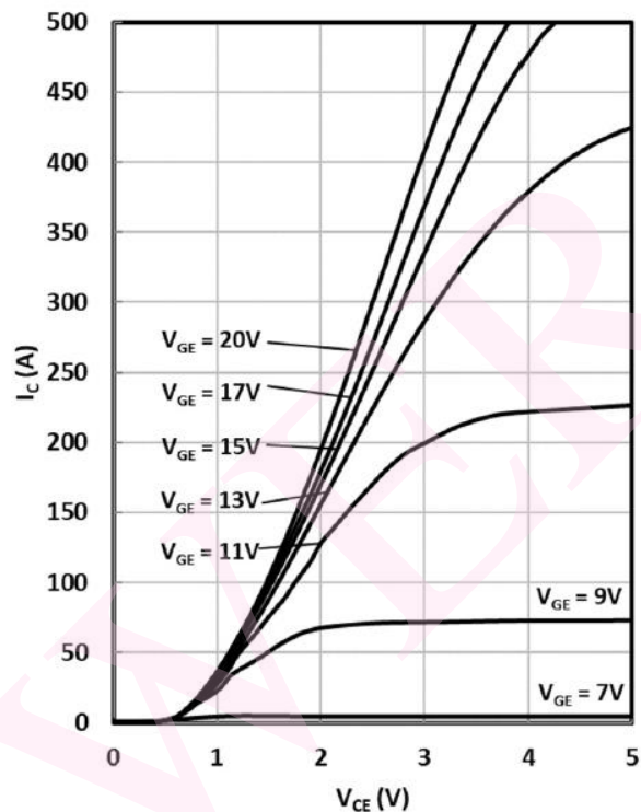
Fig. 2 IGBT (Inverter) Output Characteristics
