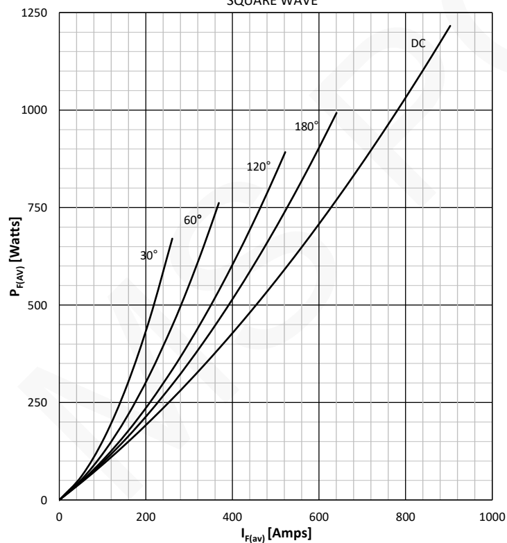
DISSIPATION CHARACTERISTICS
