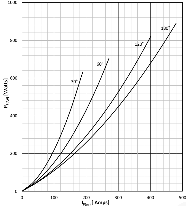
DISSIPATION CHARACTERISTICS
