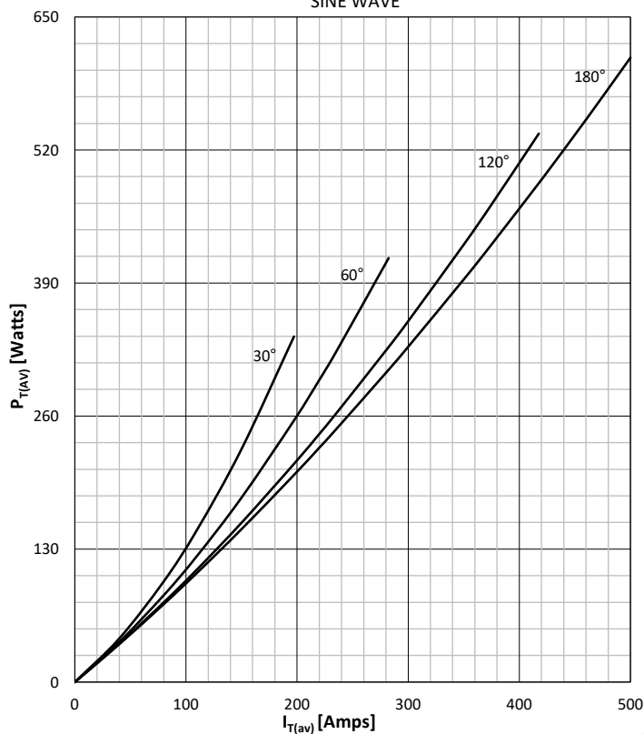
DISSIPATION CHARACTERISTICS
