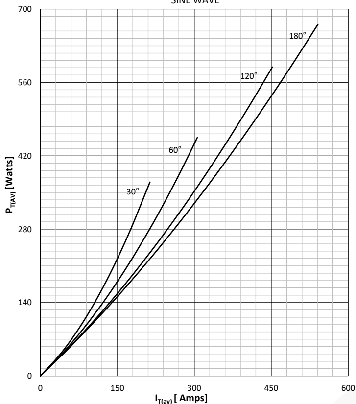
DISSIPATION CHARACTERISTICS
